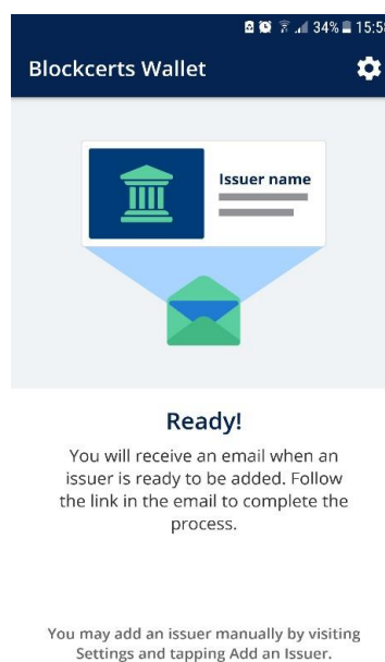
Figure 8 Final Screen
